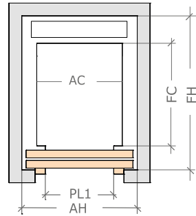
Wide-framed door detail
