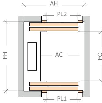
Wide-framed door detail
